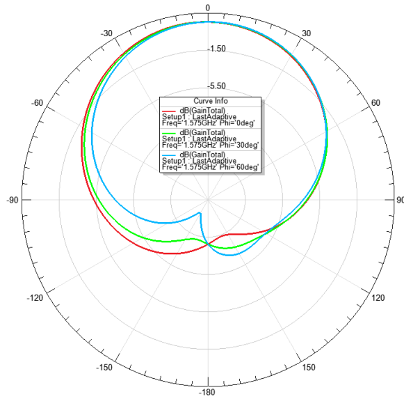
Gain Plot 2
